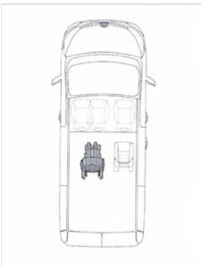
Standard conversion includes one seat in the rear and one wheelchair position
